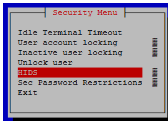
Figure 4-15 Security Menu
