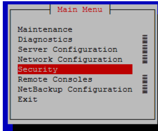
Figure 4-9 Main Menu
