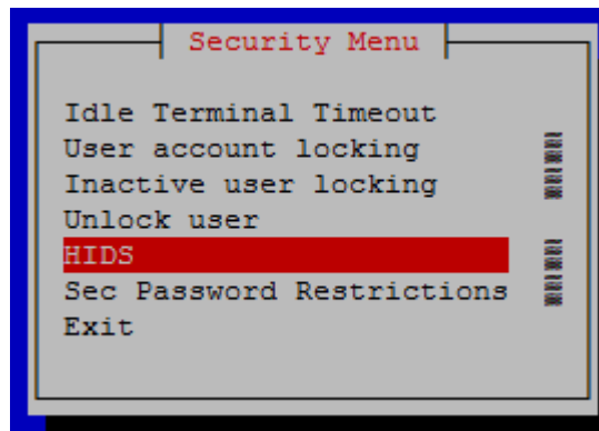
Figure 4-20 Security Menu
