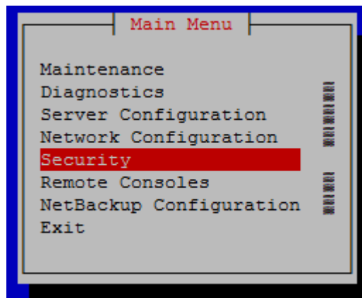
Figure 4-5 Main Menu
