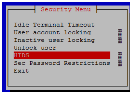
Figure 4-6 Security Menu
