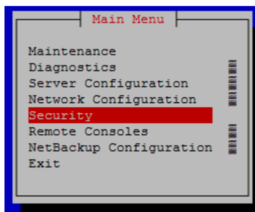
Figure 4-14 Main Menu
