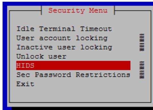
Figure 4-10 Security Menu
