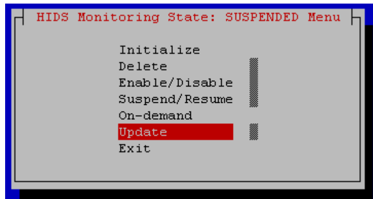
Figure 4-29 Update HIDS
