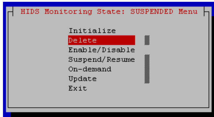
Figure 4-34 Delete HIDS
