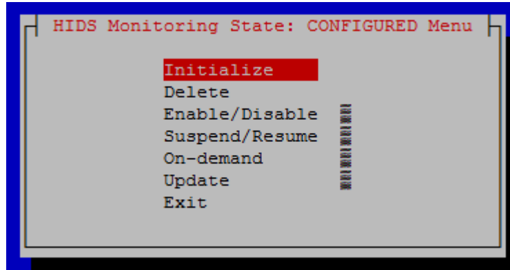
Figure 4-8 Initialize HIDS
