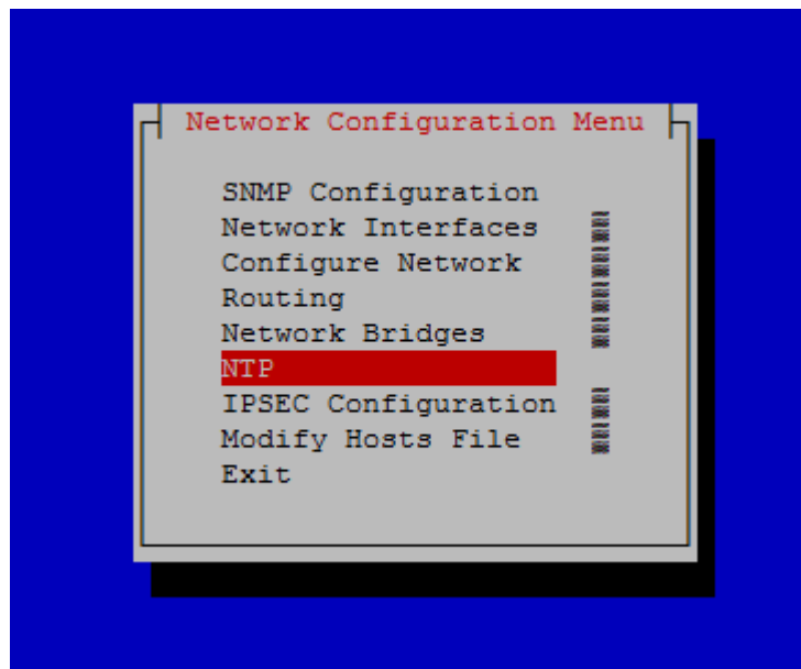
Figure 5-3 Selecting NTP
